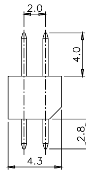
P/N:2204S-XXSG
