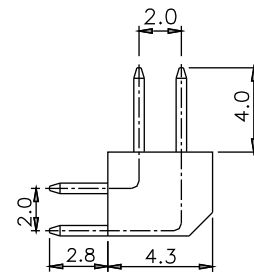
P/N:2204R-XXSG
